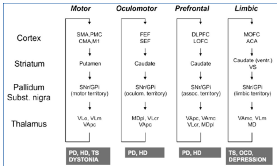
Figure 4 - Organisation anatomique en parallèle des circuits des ganglions de la base au cortex et troubles associés (d'après Alexander et al., 1990). CM, n. centre médian ; Globus pallidus externe (GPe), globus pallidus interne (GPi), noyau subthalamique (STN), substance noire pars reticulata (SNr), substantia nigra pars compacta (SNc), thalamus ventrolatéral (VL), n.ventralis anterior, pars parvocellularis (VApc), n.ventralis lateralis, pars oralis (VLo), n. medialis dorsalis pars multiformis (MDmf), paramedian pontine reticular formation (PPRF), superior colliculus (SC), n. ventralis anterior pars magnocellularis (VAmc), n. medialis dorsalis pars parvocellularis (MDpc), n. parafascicularis (Pf), N. medialis dorsalis pars magnocellularis (MDmc), ventral pallidum (VP), ventral striatum (VS), Obsessive-Compulsive Disorder (OCD), Parkinson disease (PD), Huntington's disease (HD), Tourette's syndrome (TS)..
