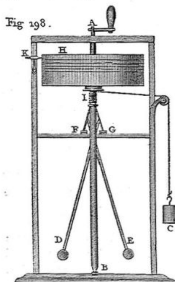
Fig 198. YOUNG'S METHOD OF RECORDING MINUTE INTERVALS OF TIME BY MEANS OF A VIBRATING STYLE WRITING ON A REVOLVING CYLINDER.
