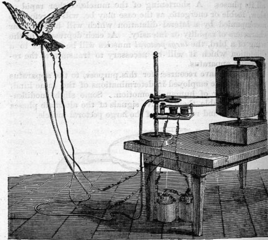
FIG. 94.—Experiment to determine by the electrical and myographical methods, at the same time, the frequency of the movements of the wing and the relative durations of its elevation and depression.
