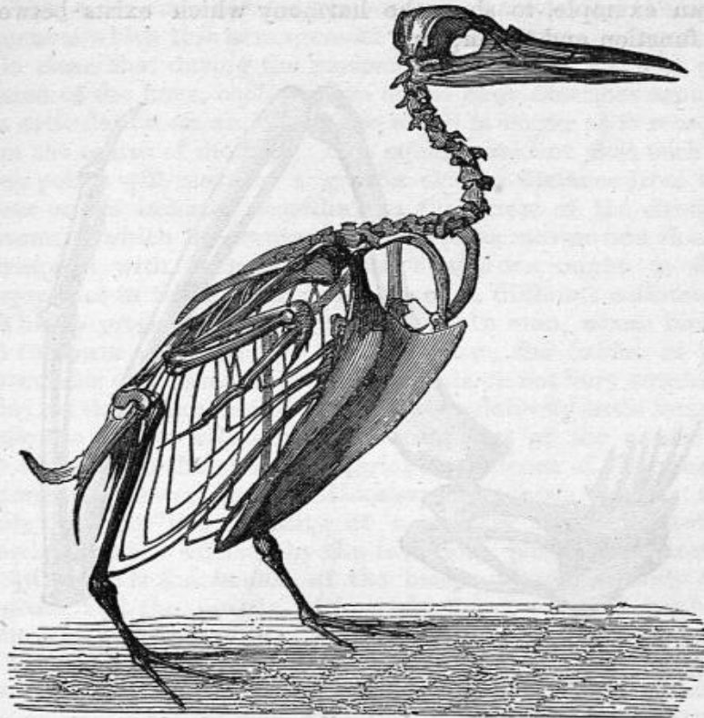
FIG. 14. —Skeleton of a penguin: sternum very long, wing very short.
