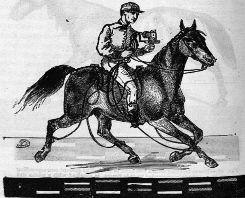
FIG. 49.—Horse at full trot. The dot placed in the notation corresponds with the attitude represented.
