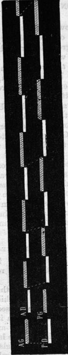
FIG. 65.— Transition from the trot to the walk.
