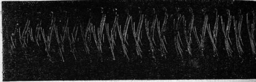
FIG. 73.—Tracing of the middle zone in the course described by the wing of a humming-bird moth. The numerous strokes of which this tracing is formed, arise from the extremity of the wing being fringed and presenting a rough surface.
