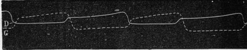
FIG. 20.—Tracings of the impact and the rise of the two feet in our ordinary walk.
