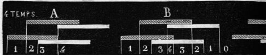
FIG. 62.—Notation of the gallop in four-time. (A) determination of each of the successive times. (B) determination of the number of feet which support the body at each instant.
