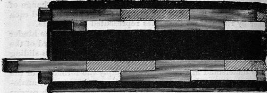
FIG. 69.—Notation rule forming the representation of the gallop in three-time.
