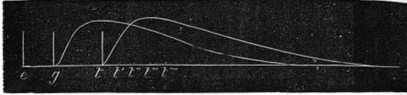
FIG. 12.—Measure of the time which elapses between the excitation of the electric nerve, and the discharge of the torpedo.
