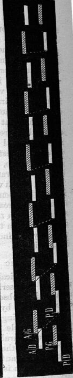
FIG. 67.— Transition from the gallop to the trot.
