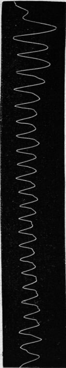
Fig. 96.—Showing the differences of amplitude and frequency of the strokes of a pigeon's wing, during a flight of 15 metres in length. To the left of the figure, we see great movements which mark the beginning of its flight. This tracing has been obtained on a cylinder whose rotation was not very rapid, which allowed us to collect a great number of movements in a small space.
