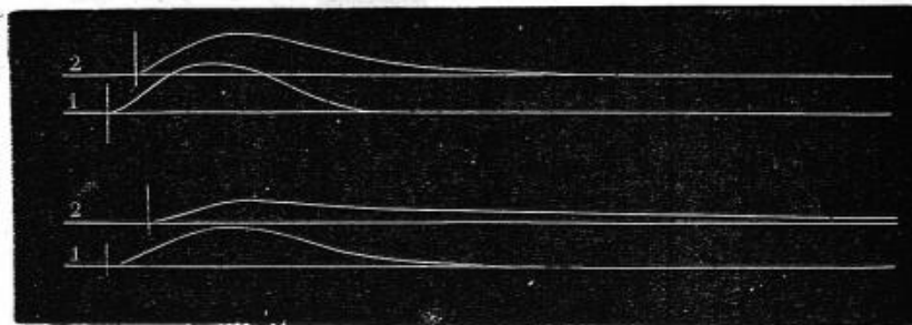
FIG. 8.—Two determinations of the speed of the muscular wave.
