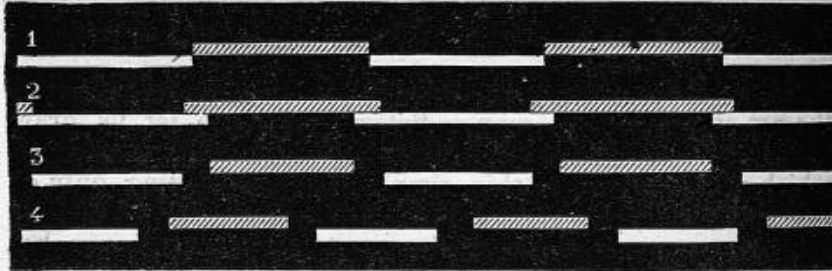
FIG. 35.—Synoptical notation of the four kinds of progression used by man.
