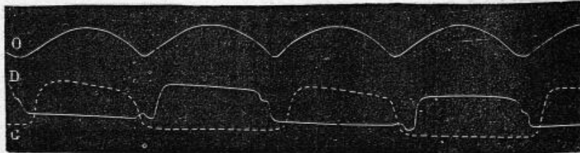
FIG. 30.—Tracing produced by running (in man). D. (curve formed by a full line), impact and rise of right foot. G. (dotted line) action of the left foot. O. oscillations and vertical re-actions of the body.
