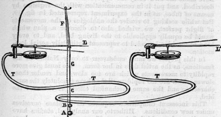
FIG. 102.—Transmission of a to-and-fro movement by means of a simple traction-cord.
