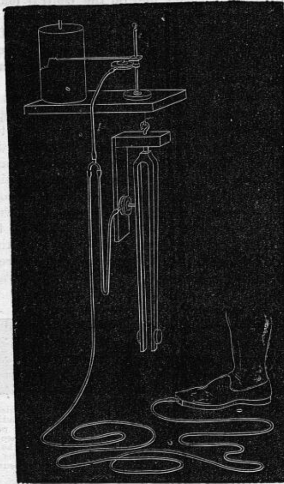
FIG. 26.—A large tuning-fork whose vibrations are reduced by masses of lead to 10 per second, acts on the registering lever drum, by an experimental drum attached to one of its branches. This also receives at the same time, by a tube with two branches, the influence both of the impact and rising of the foot of the person who walks.
