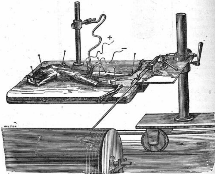
FIG. 3.—Marey's Myograph.
