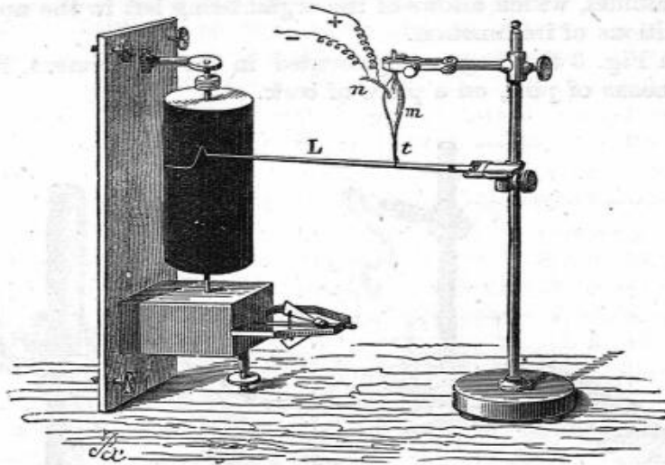
FIG. 2.—The Myograph.
