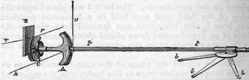
FIG. 109.—Actual arrangement of the apparatus intended to experiment upon the movements of the wing, and its change of plane.
