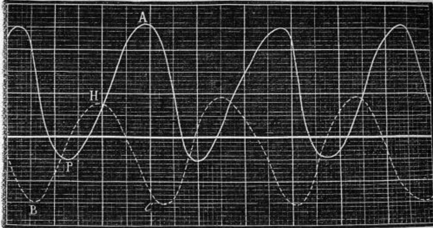
FIG. 106.—Superposition of the preceding curves on paper divided in millimetres. The two curves have a common direction with reference to the axis of the abscissæ.
