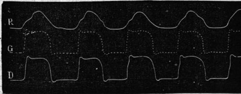
FIG. 32.—Leap on two feet at once, D and G. The line R, the curve of re-actions, shows that the maximum of elevations corresponds with the middle of the pressure of the feet.
