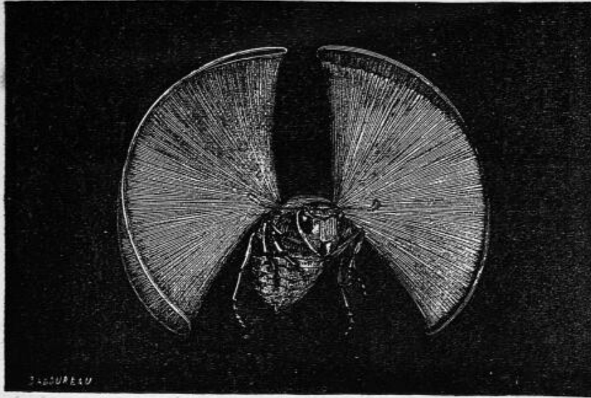
FIG. 71.—Appearance of a wasp, the extremity of each of whose larger wings has been gilded. The insect is supposed to be placed in a sun-beam.
