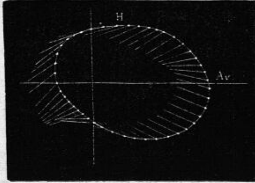
FIG. 111.—Inclinations of the plane of the wing with reference to the axis (Av) of the body during flight.
