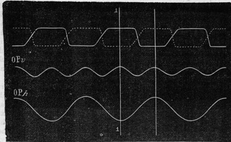
FIG. 22.—The upper curves, one in full line, the other dotted, represent the phases of the impact and of the rise of the right and left foot. Reading the figure from left to right, each rise of the curve denotes the commencement of pressure: the upper horizontal part corresponds with the duration of the pressure, and the descent with the rise of the foot. The lower horizontal part of the curve indicates that the corresponding foot is in the air. OP_v . Oscillations of the pubis from above downwards, that is, vertically, OP_h . Oscillations in a lateral direction, or horizontally. It is evident that two oscillations in the vertical direction correspond with a single horizontal oscillation.
