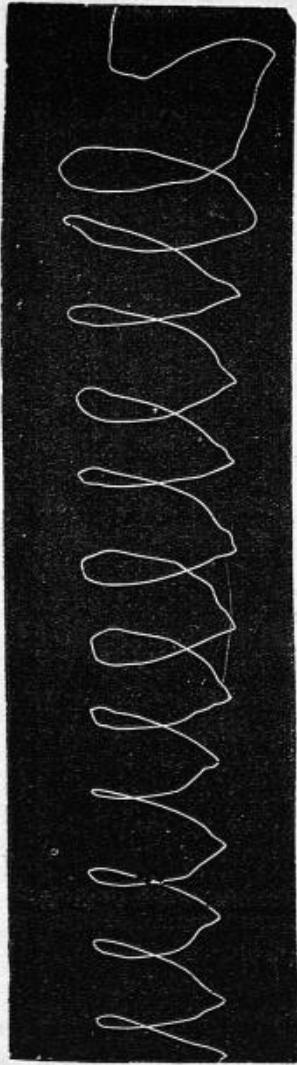
FIG. 100.—Elliptical tracing of the point of a bird's wing
