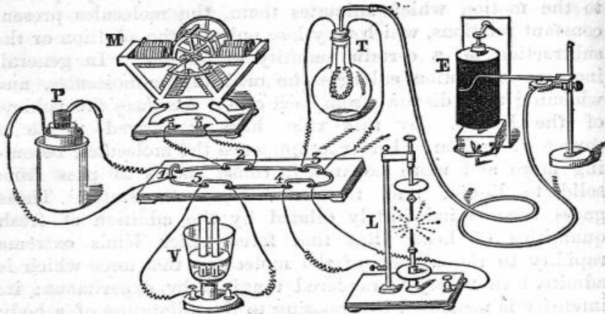
FIG. 1.—Showing the transformation of the electricity of a battery into mechanical action, into heat, light, and chemical action.
