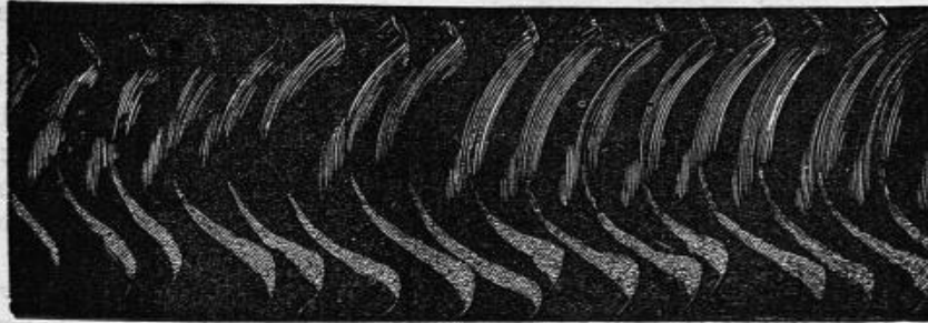
FIG. 80.—Tracings of the movements of the wing of a humming-bird moth ( macroglossa ) rubbing on the cylinder by its lower edge.
