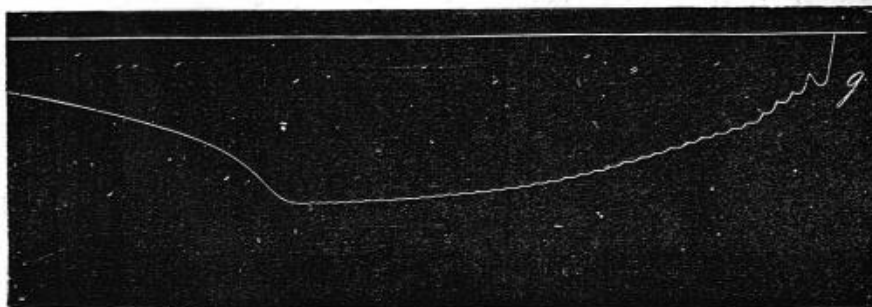
FIG. 11.—Gradual coalescence of the shocks produced by electric excitations of increasing frequency.
