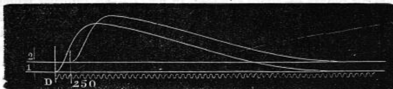
FIG. 10.—Determination of the speed of the nervous agent in man. 1. Shock produced when the nerve has been excited very close to the muscle. 2. Shock produced by the excitement of the nerve at a farther distance of 30 centimetres. D, Vibration of a chronographic tuning-fork vibrating 250 times in a second, serving to measure the time which corresponds with the interval of the shocks.
