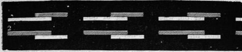
FIG. 36.—Notations of the gallop. 1. Left gallop. 2. Right gallop.
