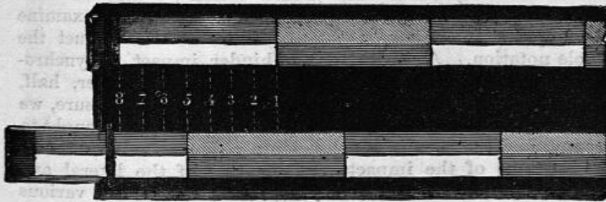
FIG. 68.—Notation rule, to represent the different paces.
