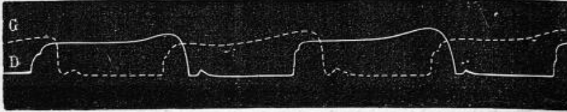
FIG. 29.—Tracing produced by walking upstairs. D. tracing of the pressure and rise of the right foot (full line). G. tracing of the left foot (dotted line). It is seen that the curves produced by the feet encroach one on the other, and that the maxima of the pressures of the feet correspond with the end of the pressures.
