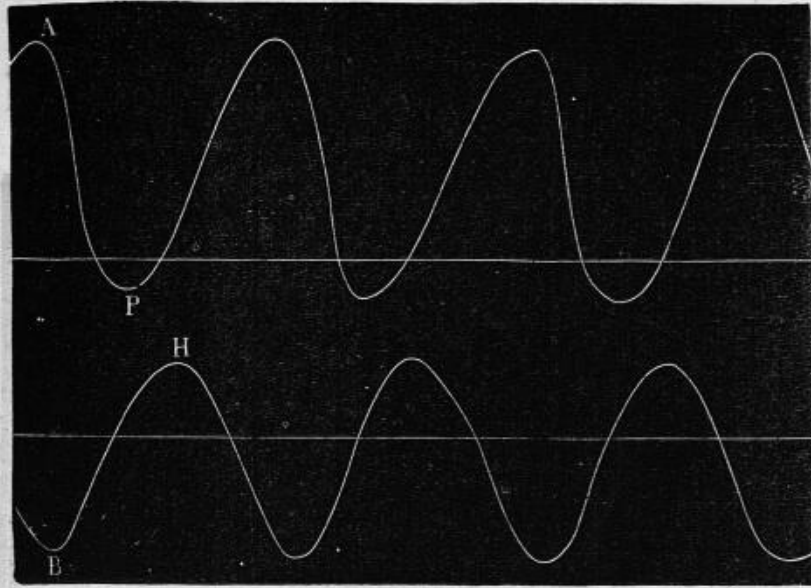
FIG. 105.—Tracing of the movements of a pigeon's wing. The upper line, A P, shows the movements forwards and backwards. The lower line H B, the movements up and down.
