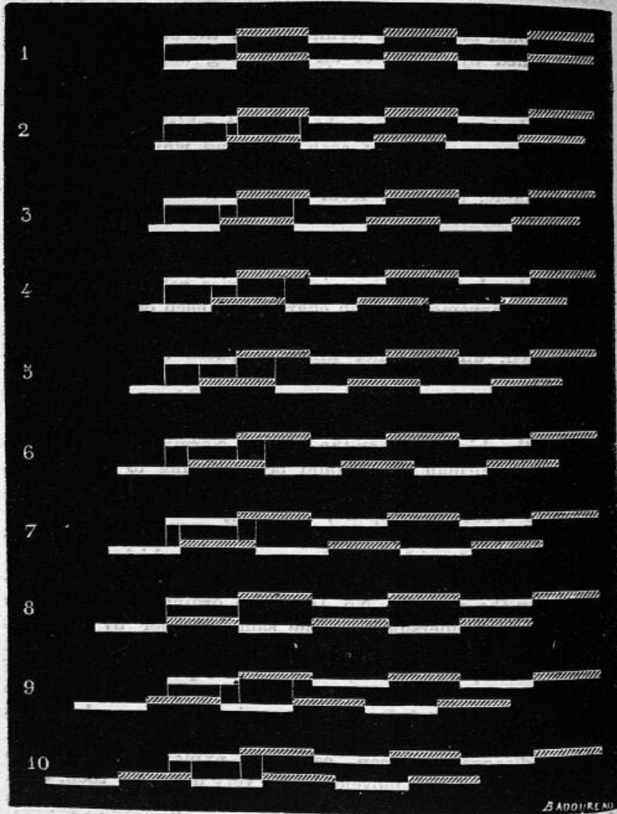
FIG. 41.—Synoptical notations of the paces of the horse, according to various writers.—See Description at the foot of page 147.
