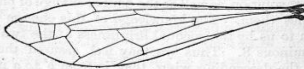
FIG. 83.—Structure of an insect's wing.
