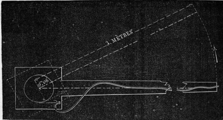
FIG. 24.—Showing two successive positions of the arm of the instrument, and the corresponding positions of the tracing points of the levers. The arm of the lever being three metres in length, and the radius of the cylinder being only six centimetres, a similar angular displacement of the person walking, and of the style which writes, will correspond with spaces which will be to each other as 50 to 1.
