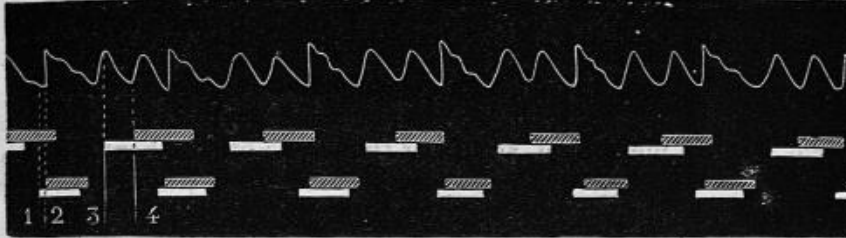
FIG. 63.—Notation of full gallop; re-actions of this pace.
