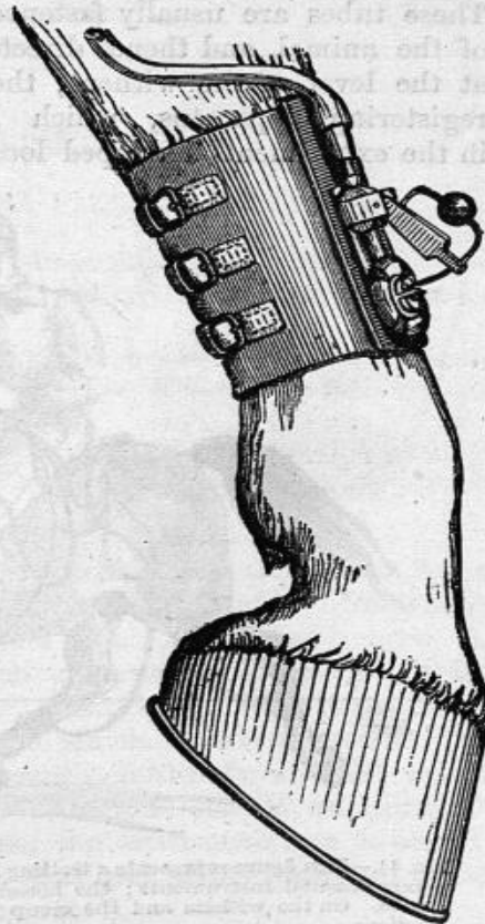
FIG. 43.—Apparatus to give the signals of the pressure and rise of the horse's hoof.
