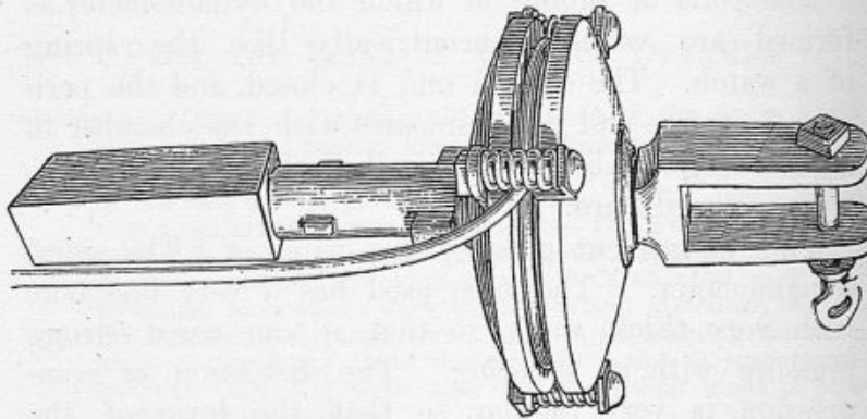
FIG. 99.—Traction dynamograph.
