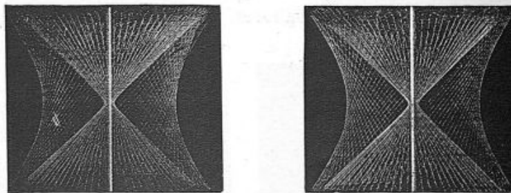
FIG. 21.—Hyperboloid and its asymptotic cone. (Stereoscopic images.)
