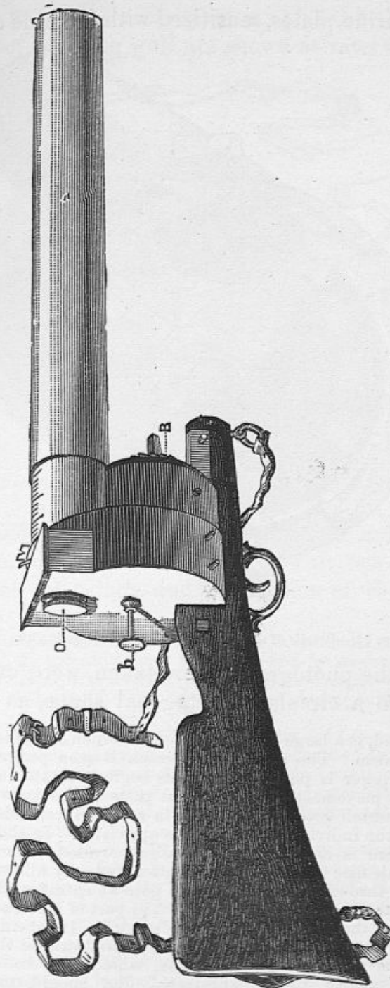
FIG. 75.—External appearance of the photographic gun.
