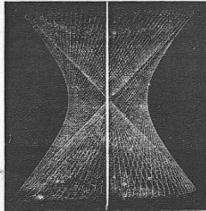
FIG. 17.—Hyperboloid by revolution with its asymptotic cone.
