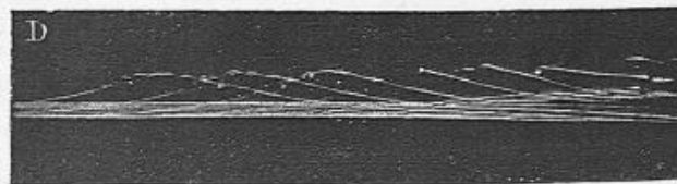
FIG. 61.—Advancing wave.
