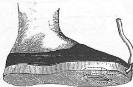
FIG. 3.—Shoe for indicating when a man's foot comes in contact with the ground; a transmitting tube effects a communication between the air chamber and the chronographic tambour.
